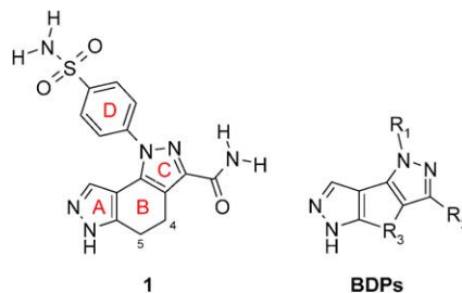
Figure 1. The structure of 1 and the general formula of BDPs.
