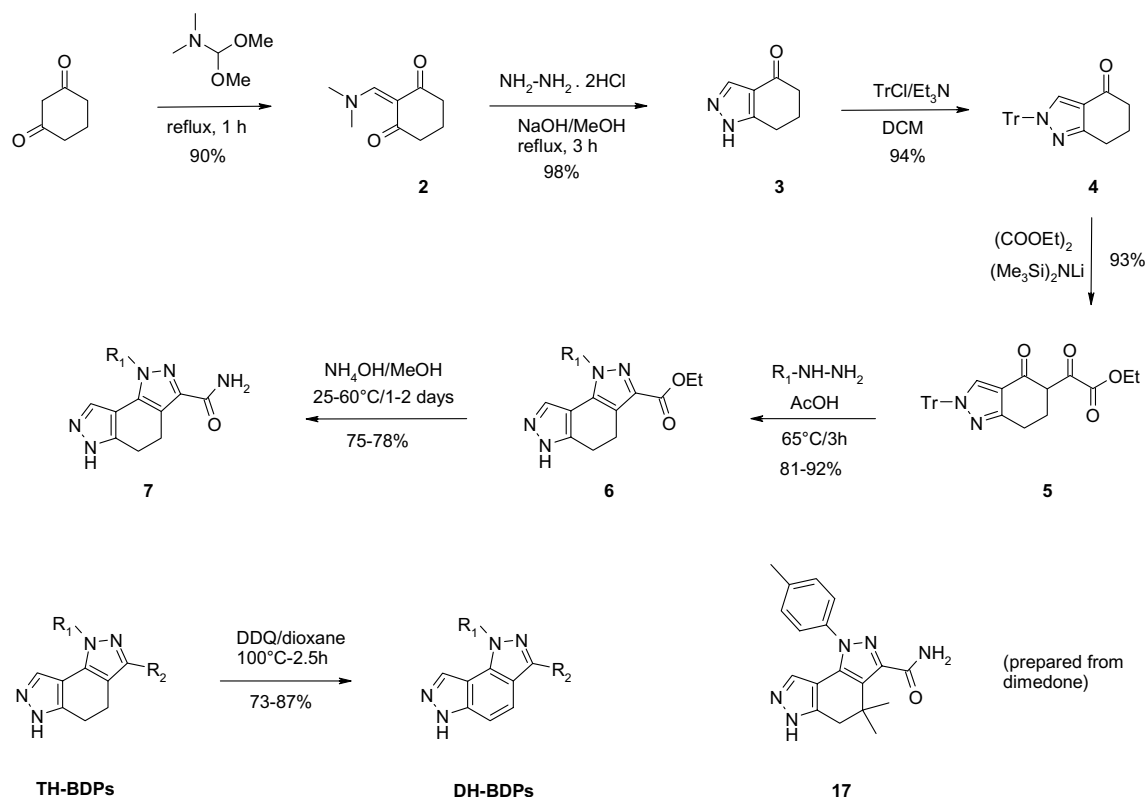
Scheme 1. General scheme for the synthesis of TH-BDPs and DH-BDPs.
