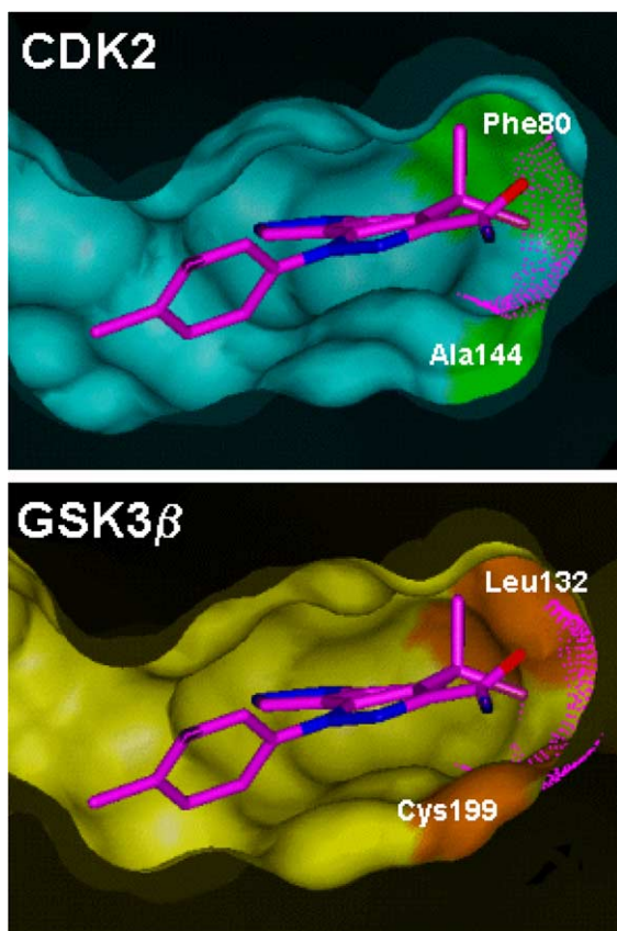
Figure 3. Compound 17 docked in CDK2 and GSK3 crystal structure.
