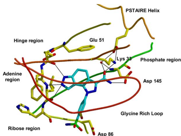
Figure 2. The crystal structure of CDK2/cyclin A in complex with compound 1 .
