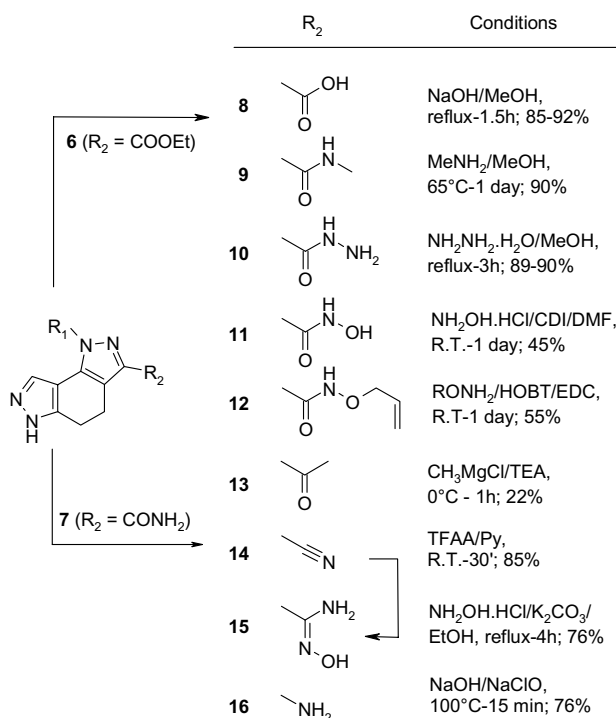
Scheme 2. Synthetic manipulations at R 2 .
